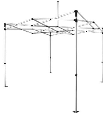
13 ft x 13 ft Professional-Grade Aluminum Actual Size: 13' x 13' x 12' Actual Weight: 80 lbs. Folded DIMs: 12" x 12" x 81" Boxed DIMs: 13" x 13" x 84" Leg: 50mm Hex
