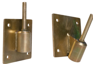
Wall Mounts - 90° and 45° 4.75" x 6.25" - 2.05 lbs.
