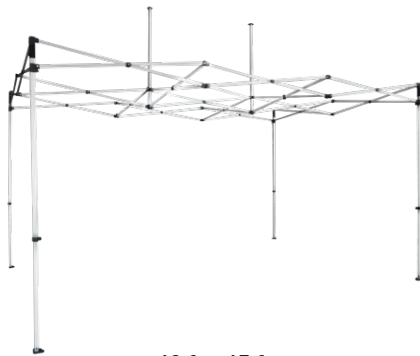
10 ft x 15 ft Commercial-Grade Steel Actual Size: 10' x 15' x 11' Actual Weight: 67 lbs. Folded DIMs: 8" x 11" x 62" Boxed DIMs: 9" x 13" x 63" Leg: 40mm Hex
