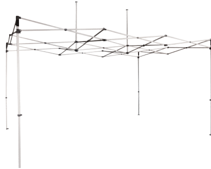
10 ft x 15 ft Commercial-Grade Aluminum Actual Size: 10' x 15' x 11' Actual Weight: 53 lbs. Folded DIMs: 9" x 15" x 62" Boxed DIMs: 10" x 13" x 63" Leg: 40mm Hex
