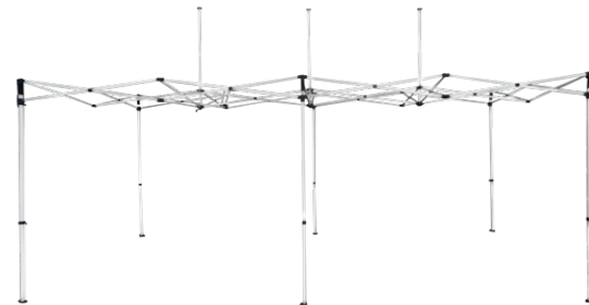
10 ft x 20 ft Commercial-Grade Steel Actual Size: 10' x 20' x 11' Actual Weight: 94 lbs. Folded DIMs: 8" x 15" x 62" Boxed DIMs: 9" x 16" x 63" Leg: 40mm Hex
