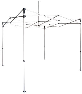
10 ft x 10 ft Commercial-Grade Aluminum Actual Size: 10' x 10' x 11' Actual Weight: 38 lbs. Folded DIMs: 9" x 9" x 62" Boxed DIMs: 10" x 10" x 63" Leg: 40mm Hex
