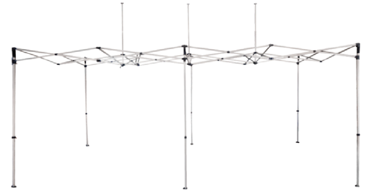
10 ft x 20 ft Commercial-Grade Aluminum Actual Size: 10' x 20' x 11' Actual Weight: 70 lbs. Folded DIMs: 9" x 16" x 62" Boxed DIMs: 10" x 17" x 63" Leg: 40mm Hex
