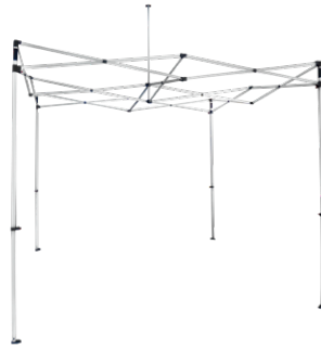
10 ft x 10 ft Lightweight Steel Actual Size: 10' x 10' x 11' Actual Weight: 48 lbs. Folded DIMs: 7" x 7" x 62" Boxed DIMs: 9" x 9" x 63" Leg: 30mm Square
