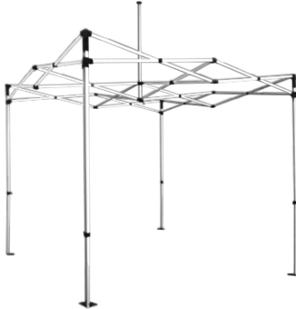
10 ft x 10 ft Professional-Grade Aluminum Actual Size: 10' x 10' x 12' Actual Weight: 61 lbs. Folded DIMs: 12" x 12" x 65" Boxed DIMs: 13" x 13" x 66" Leg: 50mm Hex
